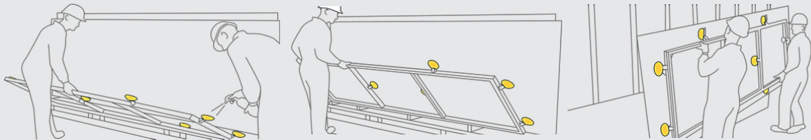
HANDLING AND SETTING OF A SLAB BY USING SUCTION FRAME
